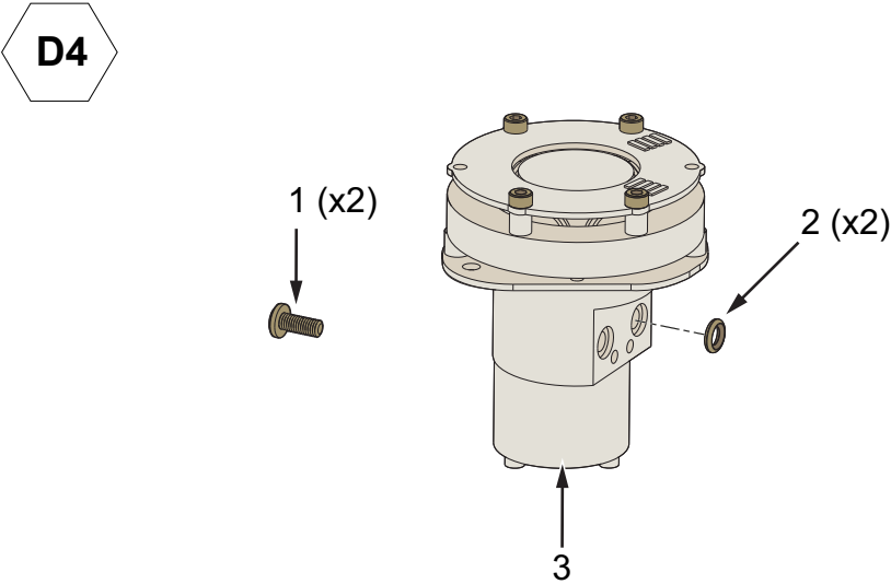
Figure 22: Ink Pump Assembly
