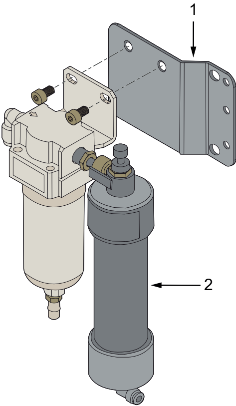
Figure 35: Air Dryer Assembly
