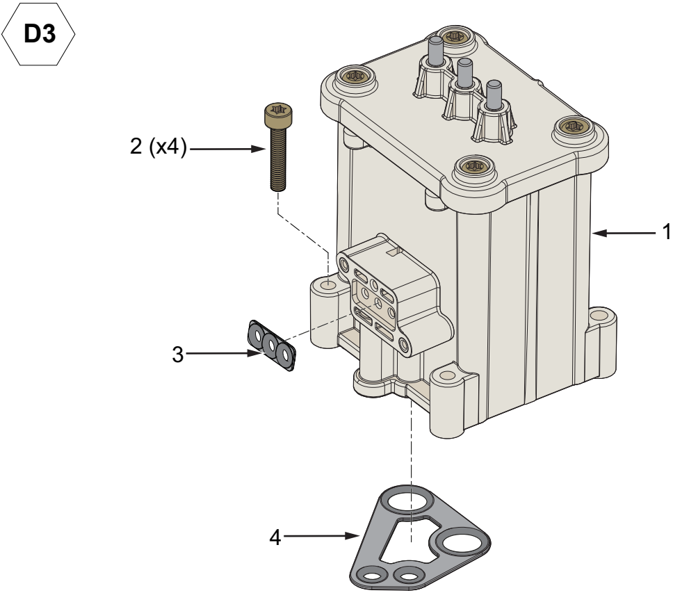
Figure 21: VMS Assembly
