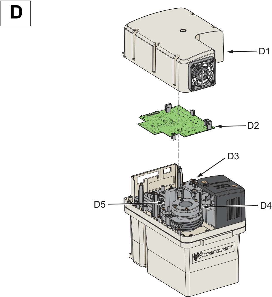
Figure 18: Ink System
