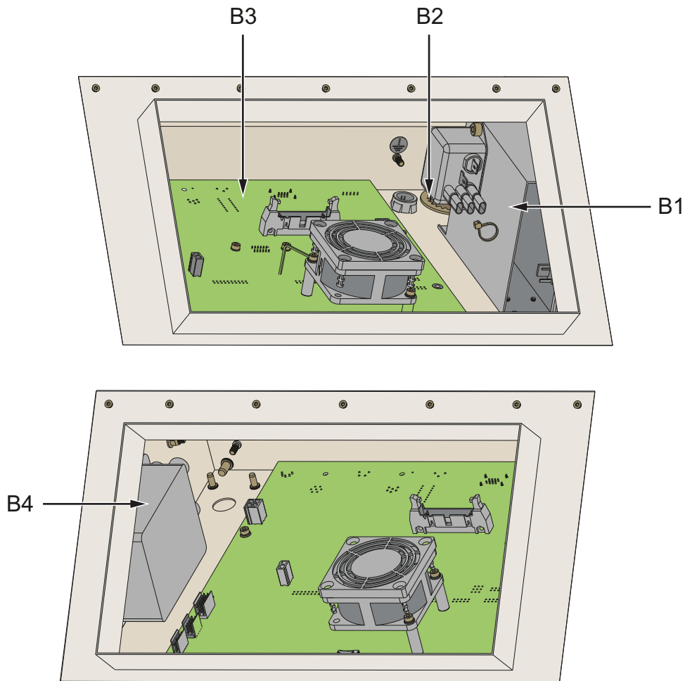
Figure 3: Electronics Compartment
