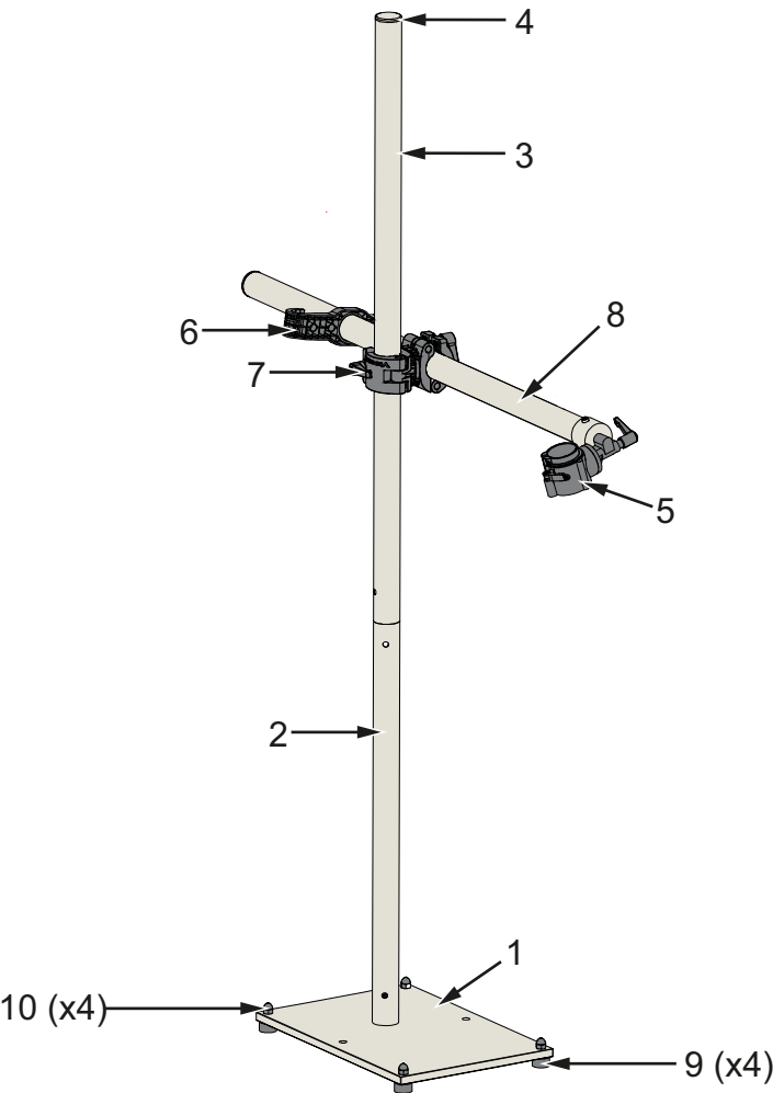
Figure 38: Printhead Stand
