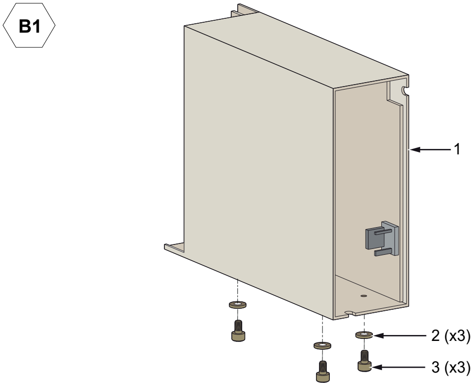
Figure 4: Main Power Supply Unit
