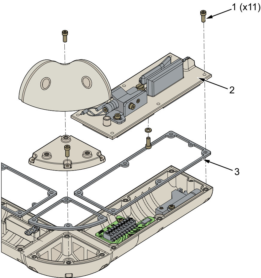
Figure 29: 90 Degree Print Module Assembly
