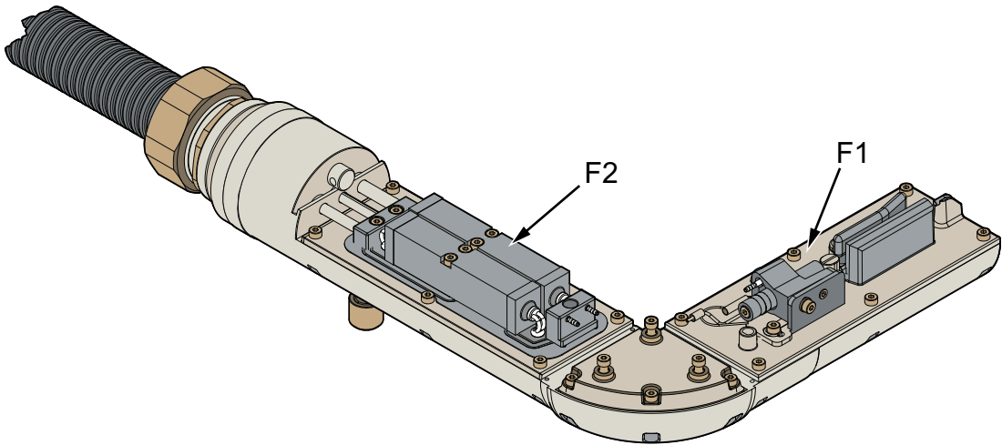
Figure 27: 90 Degree Printhead
