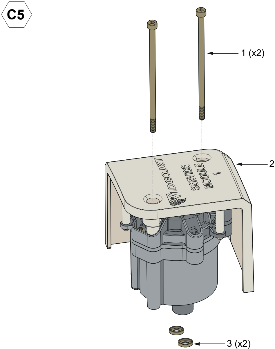
Figure 13: Service Module 1 Assembly
