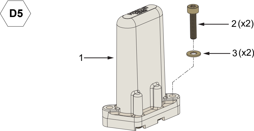
Figure 23: Pre-Venturi Filter
